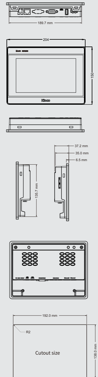
Mechanical Dimensions (Unit: mm)
