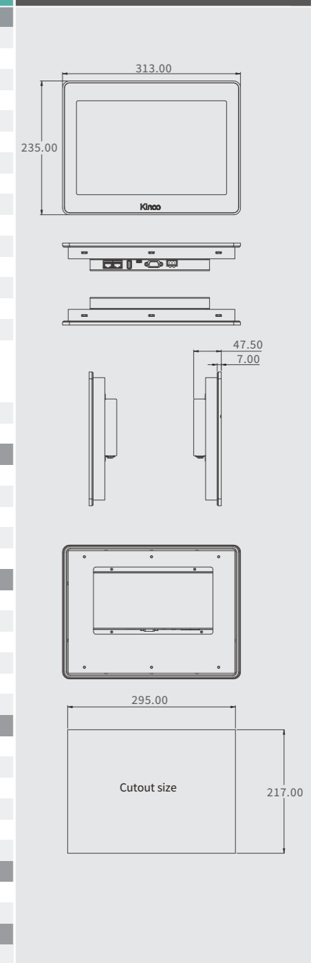
Mechanical Dimensions (Unit: mm)
