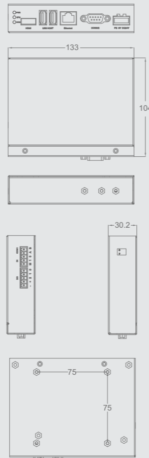
Mechanical Dimensions (Unit: mm)
